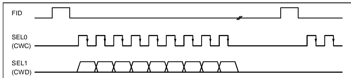
Figure 5 : PRBS Presetter
